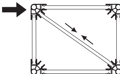
Fig. 25 - Compression acting on the strut.
