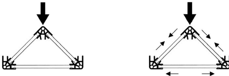
Fig. 27 - Force applied to the angle of a triangle.
