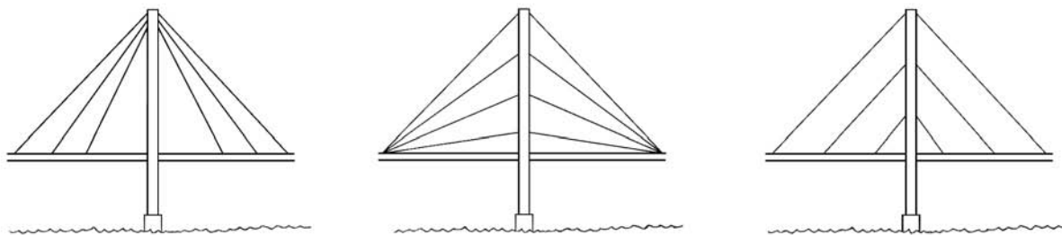
Fig. 47 - Cable designs.
